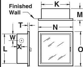
RECESSED
