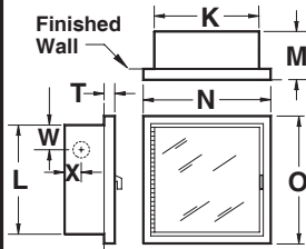
SEMI-RECESSED
